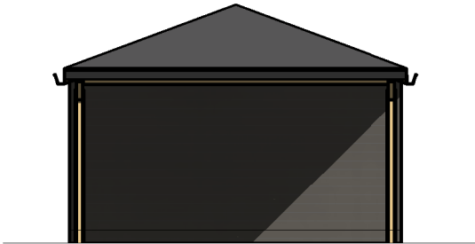
Fasade Øst-carport
